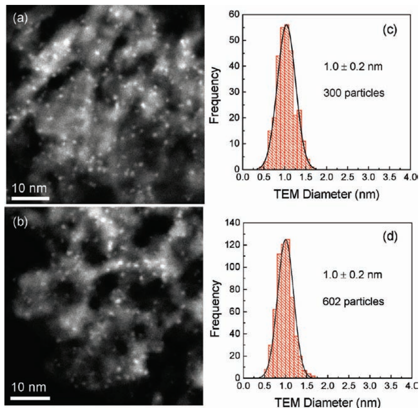
Figure 3. HAADF STEM images of micellar Pt NPs on \gamma -Al 2 O 3 : (a) S1, and (b) S2. The images were taken after polymer removal by annealing in O 2 at 375 °C. Histograms of the corresponding NP diameter distributions are shown in panels c and d.
